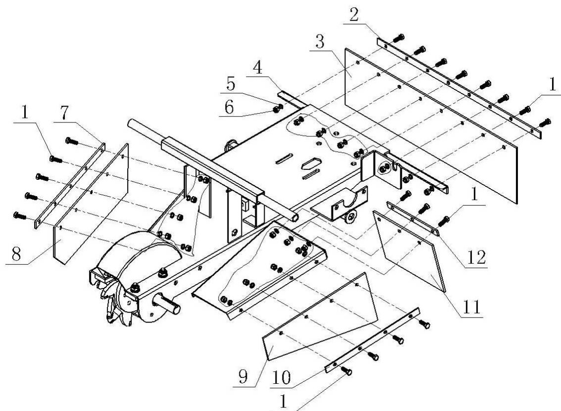
CHASSIS AND FLAP ASSY.
