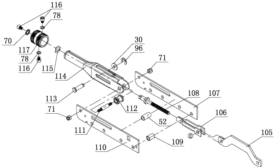
BRAKE HANDLE ASSY.
